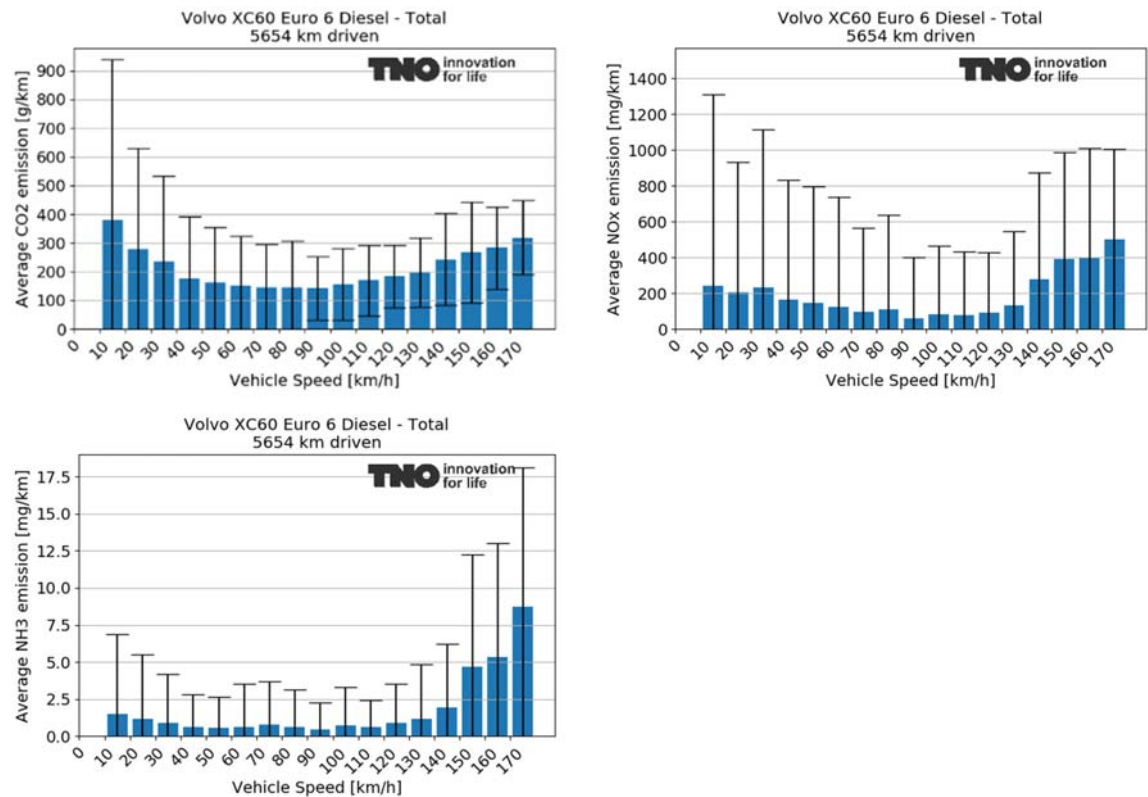
Figure A-10: Average CO 2 , NO x and NH 3 emissions dependent on vehicle speed bin during all driving for a Volvo XC 60.
