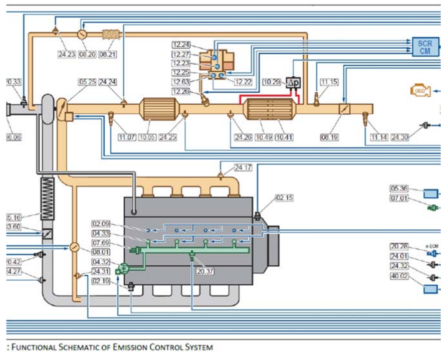
Figure A-38: Functional schematic of the Mercedes B180's emission control system (source: Mercedes-Benz Cars Nederland B.V).
