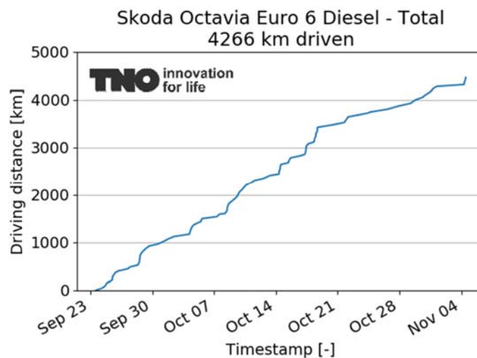
Figure A-29: Distance driven with respect to time of the test programme (in total 82.6 hours) of the Skoda Octavia.
