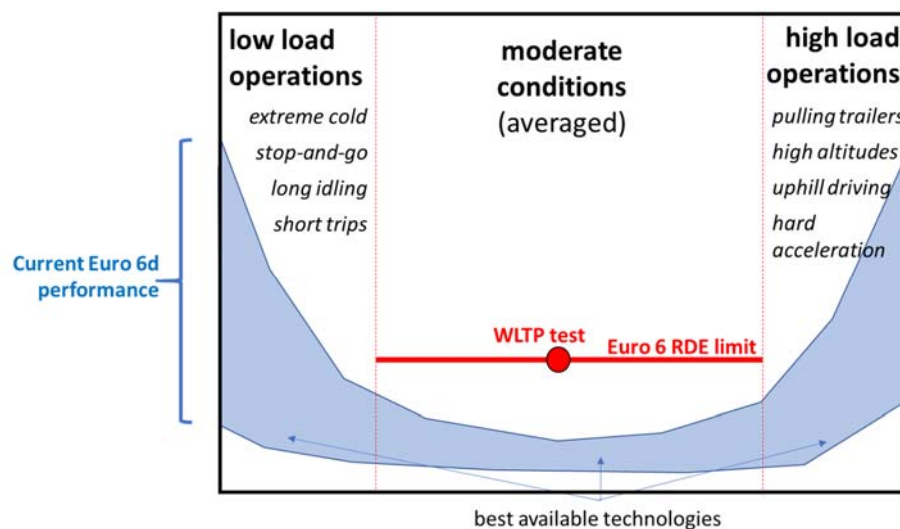
Figure 1-3: Graphic representation of current Euro 6d vehicle performance (blue band) in the context of RDE testing. The WLTP laboratory test is a very specific subset of moderate driving conditions (as indicated by the red dot). Comparatively, the RDE test addresses a much wider range of driving conditions (as shown by the red line), though these conditions could still, on average, be described as moderate. The current RDE testing procedure does not test for low load (such as extreme cold, stop-and-go traffic, long periods of idling, or short trips) or high load (e.g. pulling trailers, driving at high altitude, driving uphill, or hard acceleration) operations.
