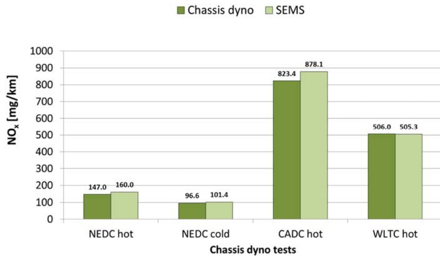
Figure A-4: NO x emissions of a Euro 6 diesel passenger car on a chassis dynamometer test: comparison of simultaneously executed measurements with the CVS/bag method of the chassis dynamometer and SEMS.
