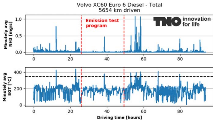
Figure A-7: NH 3 emission and exhaust gas temperatures over the test programme (in total 93.9 hours) of the Volvo XC 60. The red dotted lines mark the period of the emission test program.
