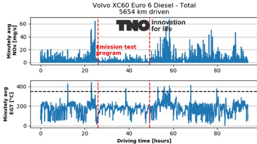
Figure A-6: NO x emission and exhaust gas temperatures over the test programme (in total 93.9 hours) of the Volvo XC 60. The red dotted lines mark the period of the emission test program.
