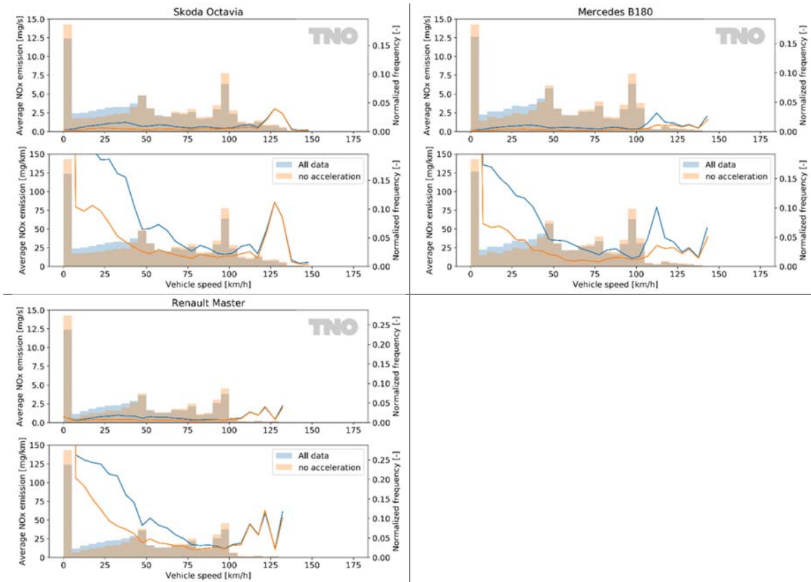
Figure 3-7: Average NO x (lines) and frequency distribution (bars) per speed bin for all data and data excluding acceleration (acceleration less than 0.5 m/s 2 , equivalent to 1.8 km/h per second).
