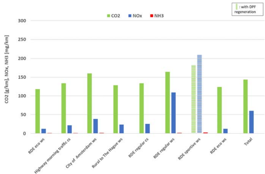
Figure A-37: Average CO 2 , NO x , NH 3 test results of the emission test programme of the Skoda Octavia
