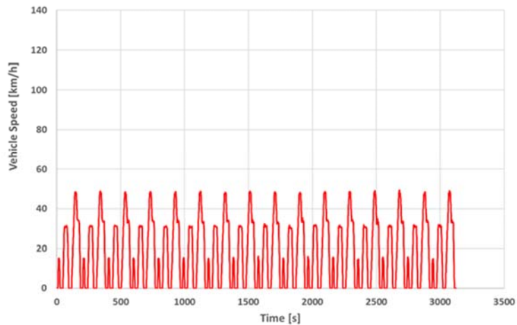
Figure A-2: 4* UDC driving test cycle.
