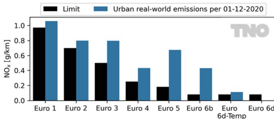
Figure 1-4: \text{NO}_x Emission factors for urban traffic and type approval limit values of Euro 1-6 diesel M1 & N1 Class 1 vehicles for the Dutch air-quality assessments (Euro 6d emission factors are not yet available).
