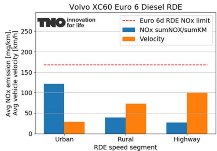
Figure A-9: Average velocities and average NOx emissions in the urban, rural and highway parts of the 'RDE' test of a Volvo XC 60.
