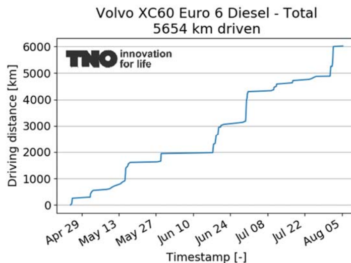
Figure A-5: Distance driven with respect to time of the test programme (in total 93,9 hours) of the Volvo XC 60.
