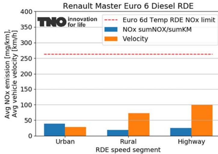
Figure A-50: Average velocities and average NO x emissions in the urban, rural and highway parts of the 'RDE' tests of a Renault Master.
