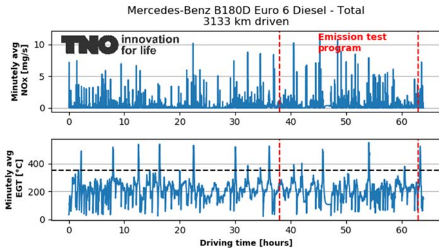
Figure A-40: NO x emission and exhaust gas temperatures over the test programme (in total 64.0 hours) of the Mercedes B180. The red dotted lines mark the period of the emission test program. The black dotted line marks the DPF regeneration threshold temperature.
