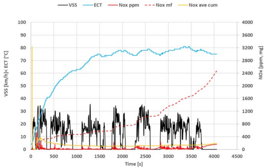
Figure A-57: Delivery trip of 66 minutes with cold start of a Euro 6d-Temp Renault Master with ambient temperatures of 0 – 3 °C. Average speed is 11.5 km/h, CO 2 367 g/km, NO x 198 mg/km.
