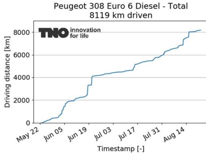
Figure A-14: Distance driven with respect to time of the test programme (in total 151.9 hours) of the Peugeot 308.
