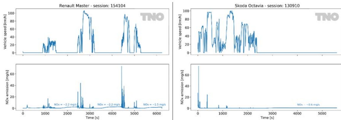
Figure 3-3: The instantaneous vehicle speed and \text{NO}_x emissions for a specific trip including extended idling for (left) the Renault Master and (right) the Skoda Octavia. Approximate \text{NO}_x levels during idling are shown via the blue annotation.
