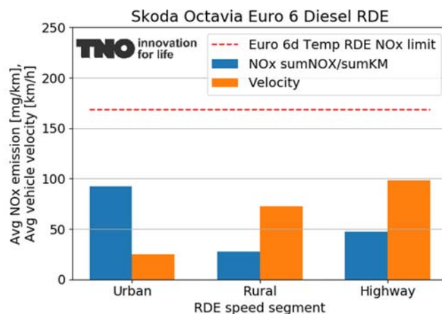
Figure A-33: Average velocities and average NO x emissions in the urban, rural and highway parts of the 'RDE' test of a Skoda Octavia.
