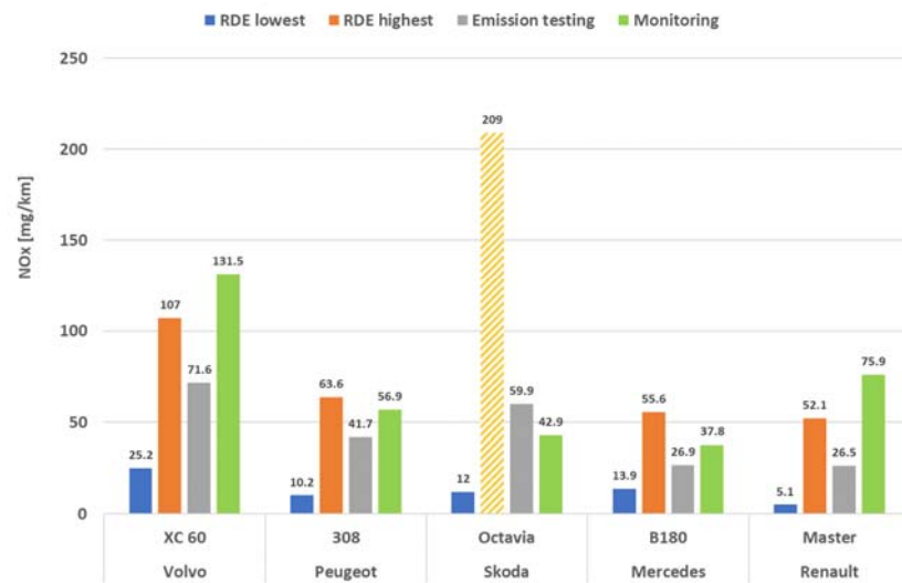
Figure A-59: NO x test results of 'RDE' tests, the emission test programme and the monitoring programme of the five tested Euro 6d-Temp diesel vehicles.
