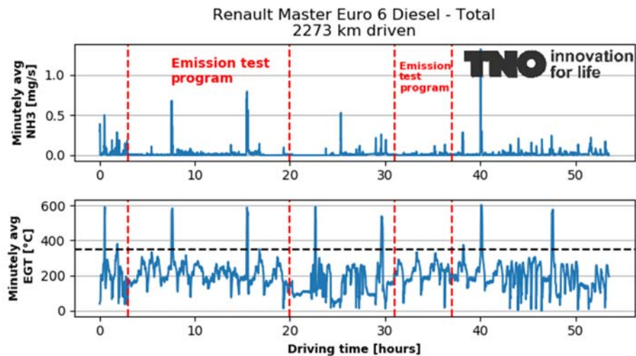
Figure A-48: NH 3 emission and exhaust gas temperatures over the test programme (in total 53.5 hours) of the Renault Master. The red dotted lines mark the period of the emission test program. The black dotted line marks the DPF regeneration threshold temperature.
