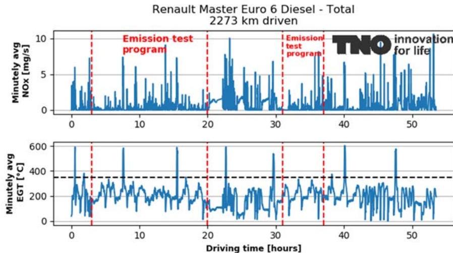
Figure A-47: NO x emission and exhaust gas temperatures over the test programme (in total 53.5 hours) of the Renault Master. The red dotted lines mark the period of the emission test program. The black dotted line marks the DPF regeneration threshold temperature.
