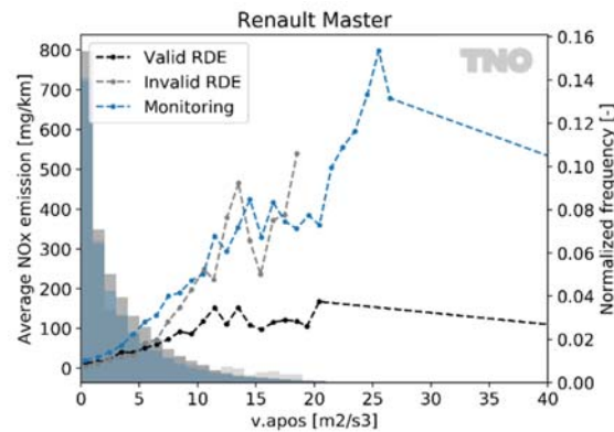
Figure 3-6: Average NOx (dashed lines with points) and frequency distribution (bars) per v \cdot a_{pos} bin for both valid and invalid RDE (black and grey) and monitoring (blue) data. Data is binned per 1 m2/s3 and is only shown if the bin has more than 20 seconds of data.
