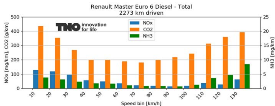
Figure A-49: Binned CO 2 , NO x and NH 3 emissions of the total test programme of the Renault Master.
