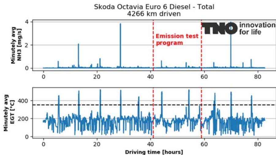
Figure A-31: NH 3 emission and exhaust gas temperatures over the test programme (in total 82.6 hours) of the Skoda Octavia. The red dotted lines mark the period of the emission test programme and the black dotted line marks the DPG regeneration threshold temperature.
