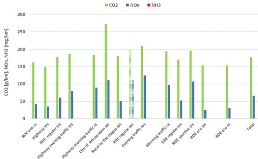
Figure A-13: Average CO 2 , NO x and NH 3 results of the emission test programme of the Volvo XC 60.
