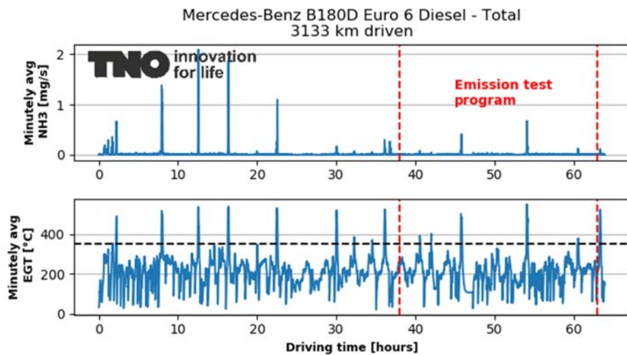
Figure A-41: NH 3 emission and exhaust gas temperatures over the test programme (in total 64.0 hours) of the Mercedes B180. The red dotted lines mark the period of the emission test program. The black dotted line marks the DPF regeneration threshold temperature.
