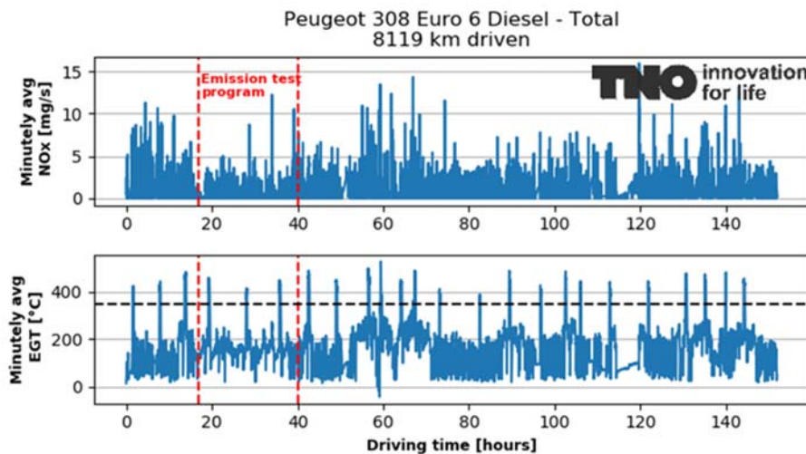
Figure A-15: NO x emission and exhaust gas temperatures over the test programme (in total 151.9 hours) of the Peugeot 308. The red dotted lines mark the period of the emission test program.
