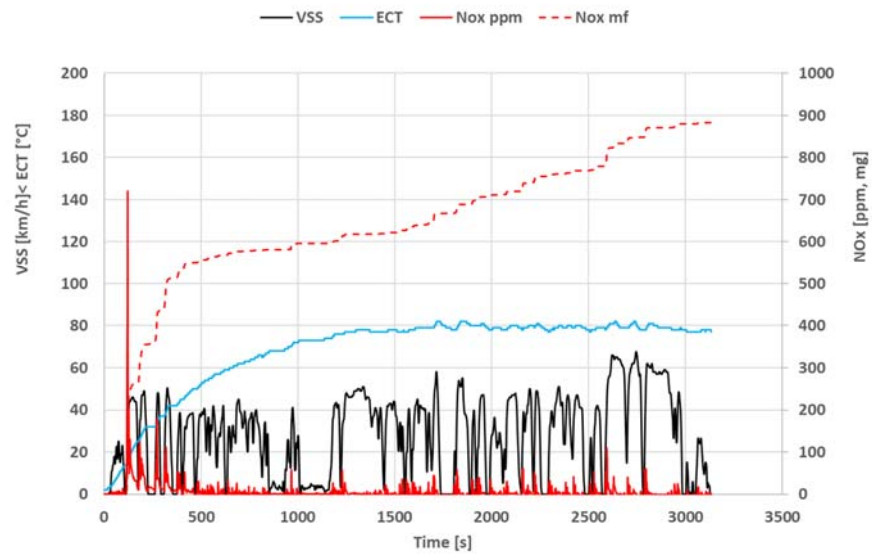
Figure A-55: Urban trip of 51 minutes with cold start of a Euro 6d-Temp Renault Master with ambient temperatures of 0 – 3 °C. Average speed is 27.9 km/h, CO 2 256 g/km, NO x 37 mg/km.
