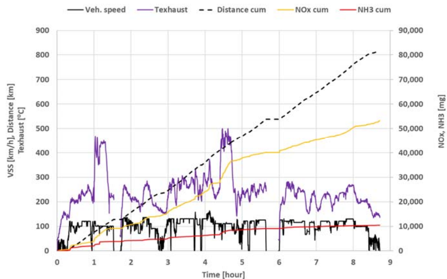
Figure A-28: Example of a long haul trip from Switzerland to The Netherlands (815 km, average vehicle speed 99.4 km/h). The average emissions were CO 2 133 g/km, NO x 65 mg/k0m and NH 3 13 mg/km. The DPF was regenerated two times during 20 minutes, the interval was 333 km).
