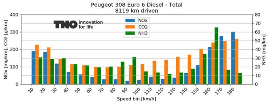
Figure A-18: Binned CO 2 , NO x and NH 3 emissions of the total test programme of the Peugeot 308.
