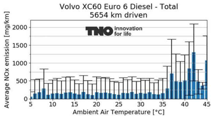
Figure A-11: Average NO x emissions per ambient air temperature bin during all driving for a Volvo XC 60. Note that the ambient air temperature is logged by the vehicle, and therefore can be affected by the state of the vehicle itself. Furthermore, this does not address the respective driving situations at these temperatures (i.e. driving behaviour can be different in summer due to a range of factors, let alone the temperature).
