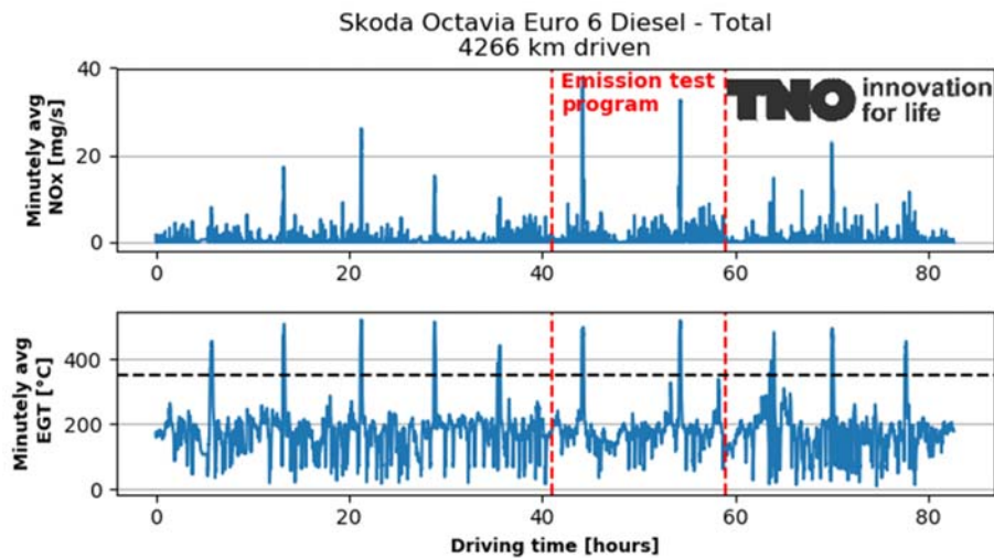
Figure A-30: NO x emission and exhaust gas temperatures over the test programme (in total 82.6 hours) of the Skoda Octavia. The red dotted lines mark the period of the emission test programme and the black dotted line marks the DPG regeneration threshold temperature.
