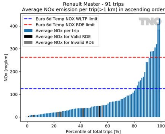
Figure 3-1: Average NO x emissions per trip for every trip driven by the five 6d-Temp vehicles, as sorted by increasing average NO x . The valid RDE trips are indicated by the black bars, while the invalid RDE trips are grey. The invalid RDE trips include, for example, the RDE trips with DPF regenerations, especially in the case of the Skoda (see also Appendix A). The WLTP and RDE limit are indicated by the blue and red dashed lines respectively.
