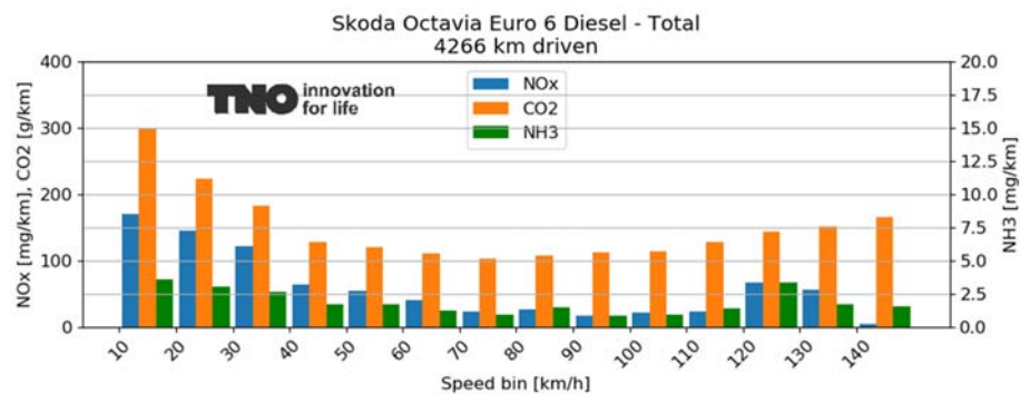
Figure A-32: Binned CO 2 , NO x and NH 3 emissions of the total test programme of the Skoda Octavia.
