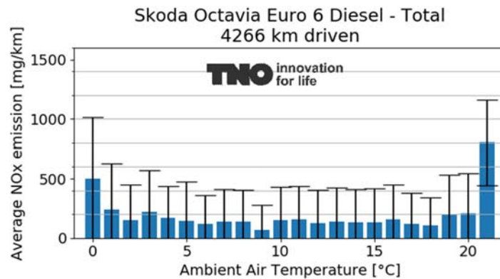
Figure A-35: Average NO x emissions per ambient air temperature bin during all driving for a Skoda Octavia. Note that the ambient air temperature is logged by the vehicle, and therefore can be affected by the state of the vehicle itself. Furthermore, this does not address the respective driving situations at these temperatures (i.e. driving behaviour can be different in summer due to a range of factors, let alone the temperature).
