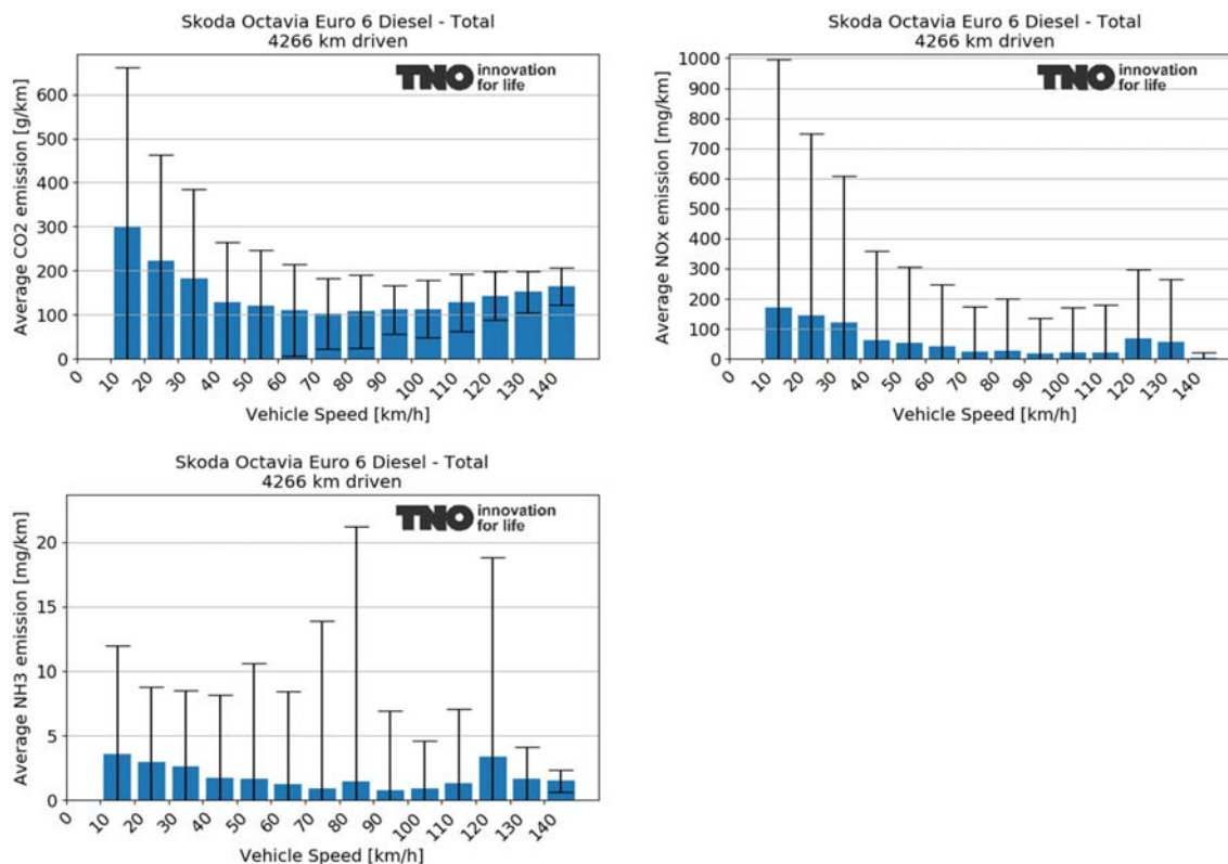
Figure A-34: Average CO 2 , NO x and NH 3 emissions dependent on vehicle speed bin during all driving for a Skoda Octavia.
