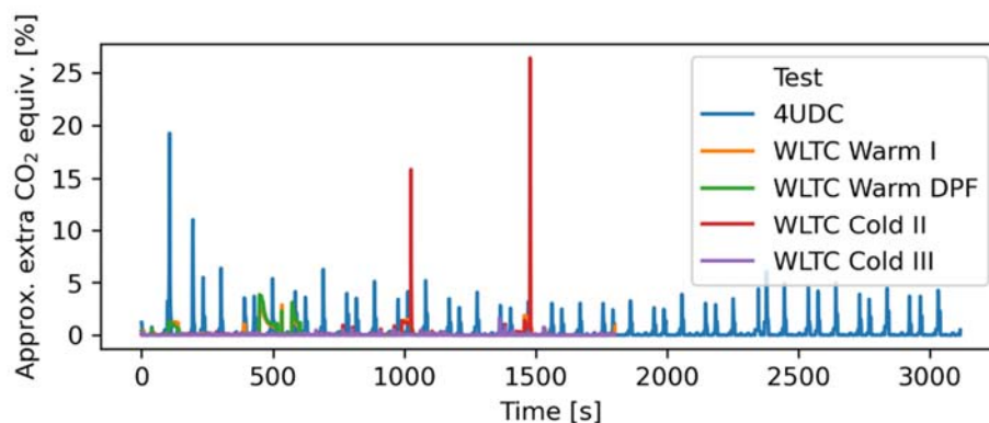
Figure 4-4: Approximate extra CO 2 equivalents of N 2 O over time for each of the chassis dynamometer tests where N 2 O was measured.
