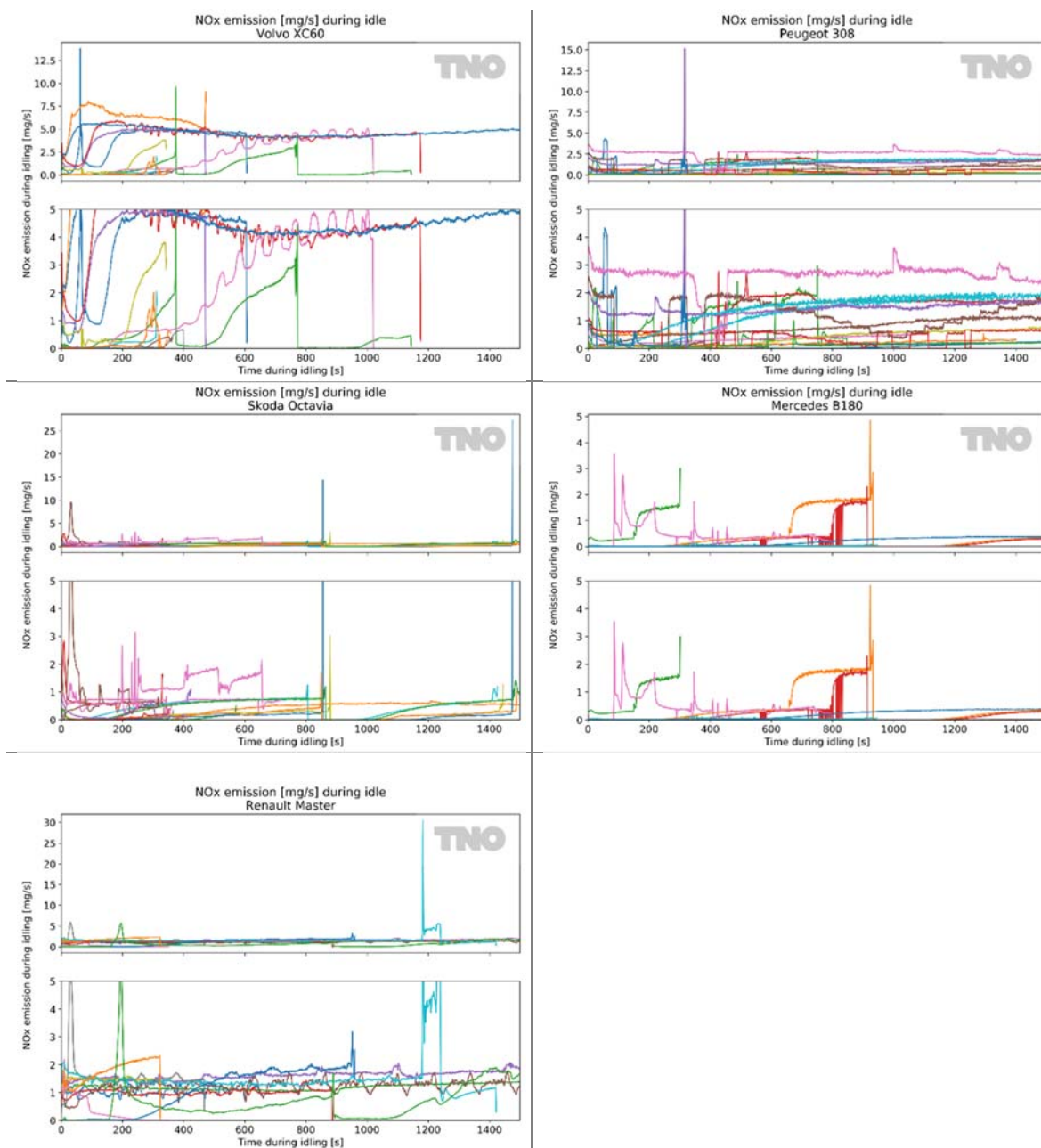
Figure 3-4: Instantaneous NO x emissions after idling has started, for all periods of extended idling. These periods are defined as when the vehicle speed is less than 5 km/h for at least 300 s. The y-axis in the top frame per vehicle is scaled automatically to show all data, while the bottom frame per vehicle shows emissions 0 – 5 mg/s.
