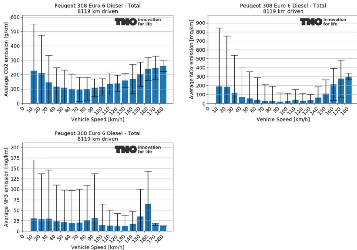
Figure A-17: Average CO 2 , NO x and NH 3 emissions dependent on vehicle speed bin during all driving for a Peugeot 308.
