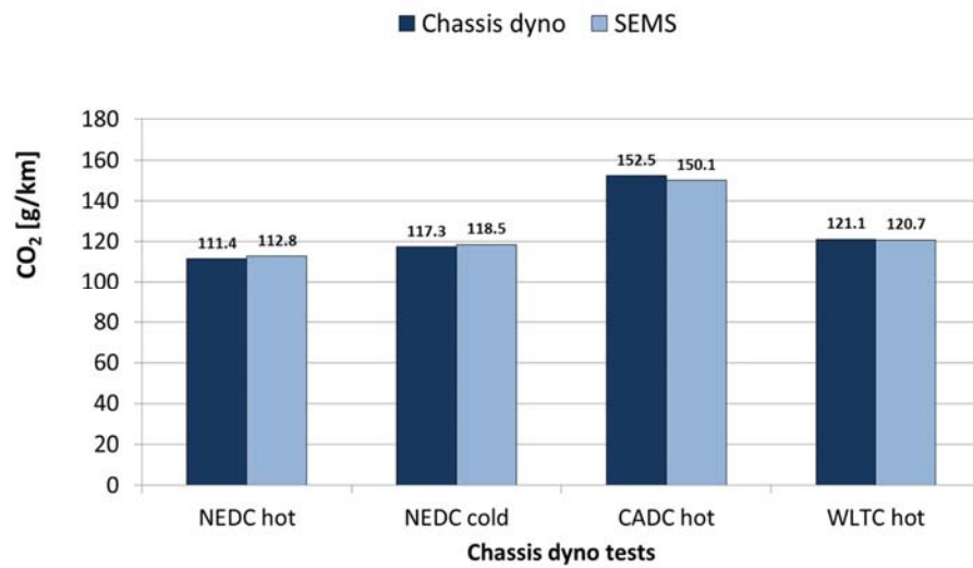
Figure A-3: CO 2 emissions of a Euro 6 diesel passenger car on a chassis dynamometer test: comparison of simultaneously executed measurements with the CVS/bag method of the chassis dynamometer and SEMS.
