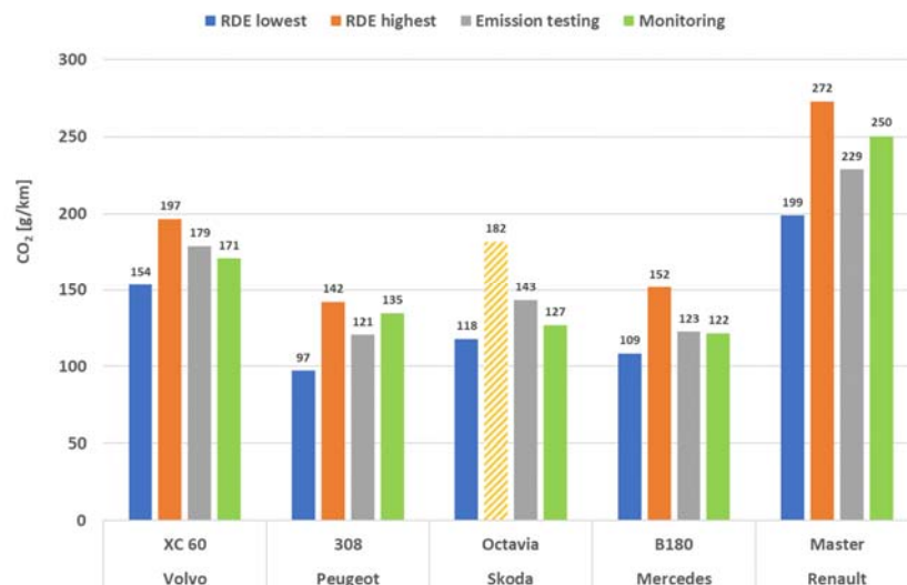
Figure A-58: CO 2 test results of 'RDE' tests, the emission test programme and the monitoring programme of the five tested Euro 6d-Temp diesel vehicles.
