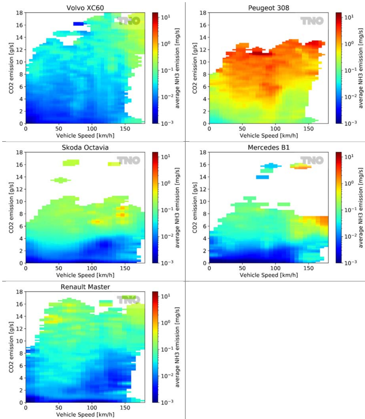
Figure 4-3: Two-dimensional emission map of average \text{NH}_3 emissions shown dependent on \text{CO}_2 emissions and vehicle speed.
