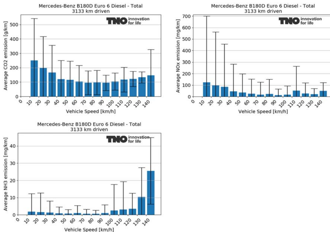
Figure A-44: Average CO 2 , NO x and NH 3 emissions dependent on vehicle speed bin during all driving for a Mercedes B180
