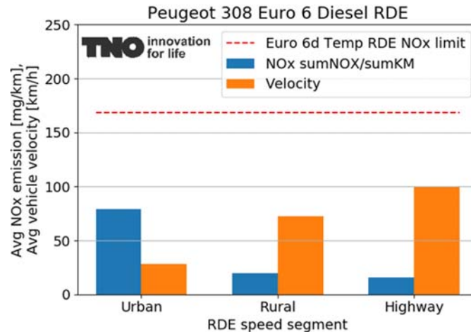
Figure A-19: Average velocities and average NO x emissions in the urban, rural and highway parts of the 'RDE' test of a Peugeot 308.
