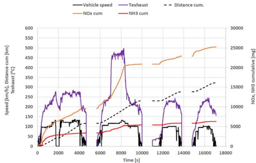
Figure A-27: Four motorway trips (total distance 321.7 km). In the second trip the duration of the DPF regeneration at vehicle speeds of 115 to 130 km/h was 21 minutes.
