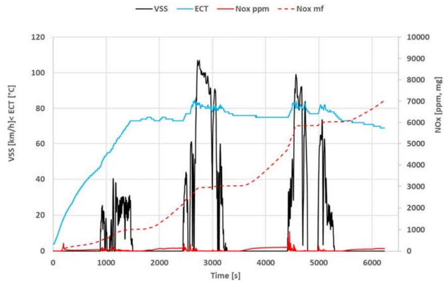
Figure A-56: Trip of 105 minutes with cold start and idling periods of a Euro 6d-Temp Renault Master with ambient temperatures of 1 – 7 °C. Average speed is 14.4 km/h, CO 2 352 g/km, NO x 287 mg/km.
