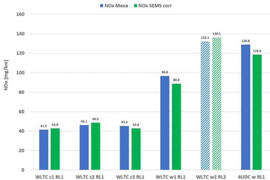
Figure A-25: WLTC and UDC NO x test results of a Peugeot Euro 6d-Temp diesel measured with CVS and SEMS. In the WLTC w2 RL2 test the DPF was regenerated.
