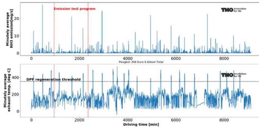
Figure A-22: Minutely average NH 3 emissions and exhaust gas temperature of the Peugeot 308 over all measurement data.
