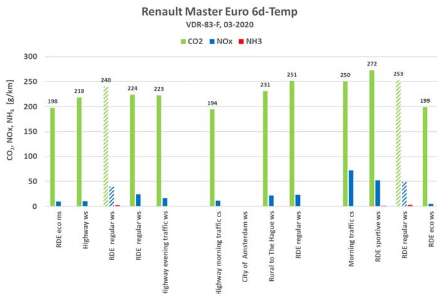
Figure A-54: Average CO 2 , NO x , NH 3 results of the emission test programme of the Renault Master.
