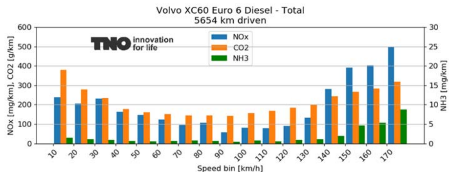
Figure A-8: Binned CO 2 , NO x and NH 3 emissions of the total test programme of the Volvo XC 60.
