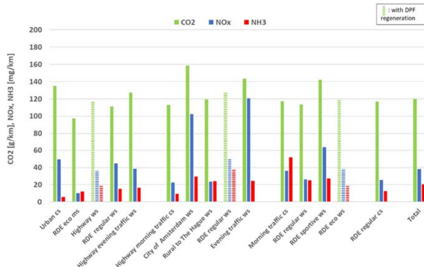
Figure A-23: Test results of the emission test programme of the Peugeot 308.
