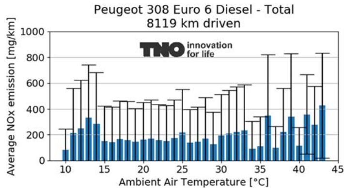
Figure A-20: Average NO x emissions per ambient air temperature bin during all driving for a Peugeot 308. Note that the ambient air temperature is logged by the vehicle, and therefore can be affected by the state of the vehicle itself. Furthermore, this does not address the respective driving situations at these temperatures (i.e. driving behaviour can be different in summer due to a range of factors, let alone the temperature).
