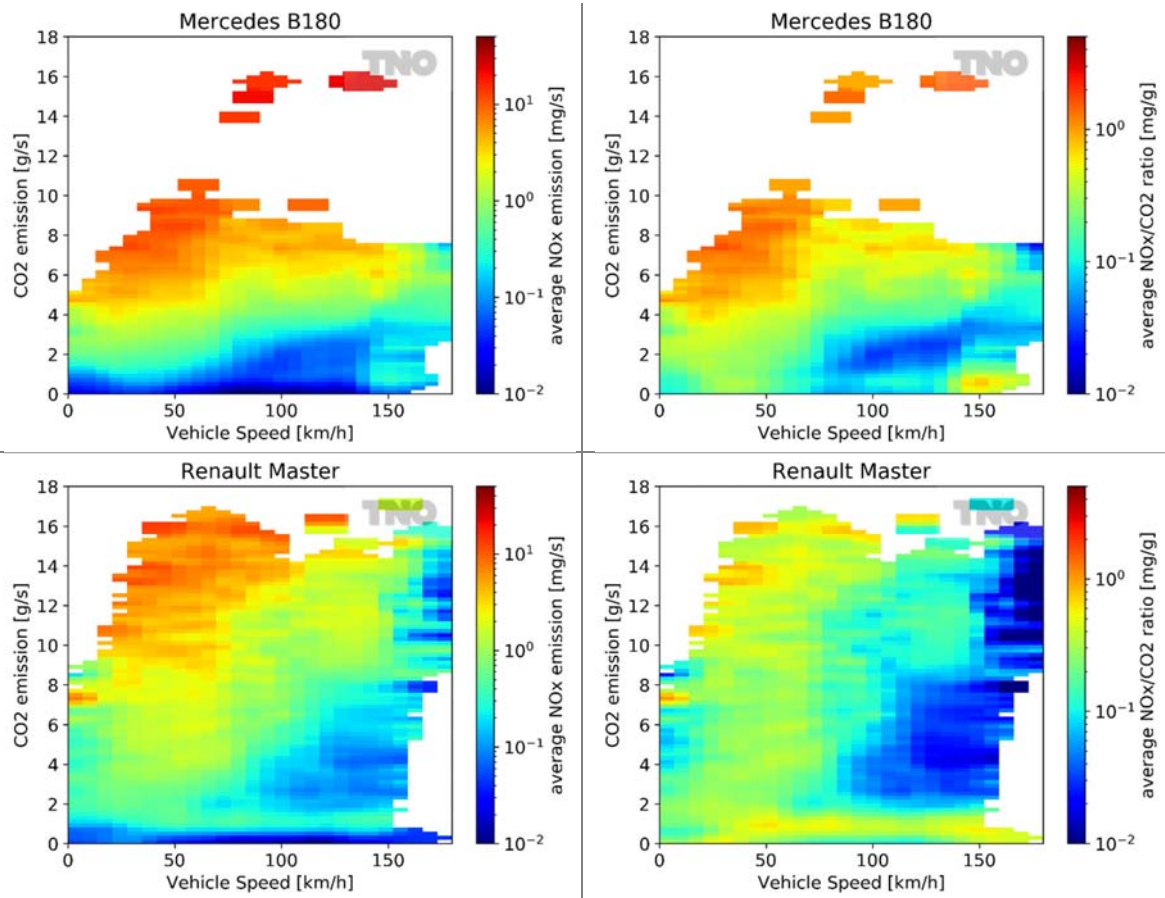
Figure 3-8: Two-dimensional emission map of average NO x emissions (left) and average NO x /CO 2 ratio (right), both shown dependent on CO 2 emissions and vehicle speed.
