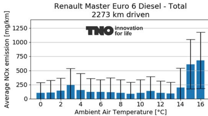
Figure A-52: Average NO x emissions per ambient air temperature bin during all driving for a Renault Master. Note that the ambient air temperature is logged by the vehicle, and therefore can be affected by the state of the vehicle itself. Furthermore, this does not address the respective driving situations at these temperatures (i.e. driving behaviour can be different in summer due to a range of factors, let alone the temperature).
