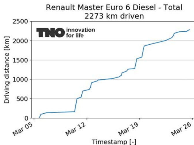
Figure A-46: Distance driven with respect to time of the test programme (in total 53.5 hours) of the Renault Master.
