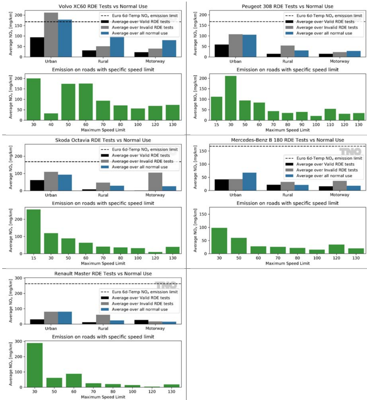
Figure 3-2: Average NO x emissions per RDE speed section for the valid and invalid RDE trips (black and grey bars) and for all normal use/monitoring (blue bars), as compared to emissions on roads with specific speed limits (green bars). Note that speed limits are only shown if the respective vehicle has spent more than 15 min on roads with that limit.
