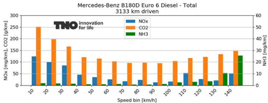
Figure A-42: Binned CO 2 , NO x and NH 3 emissions of the total test programme of the Mercedes B180.
