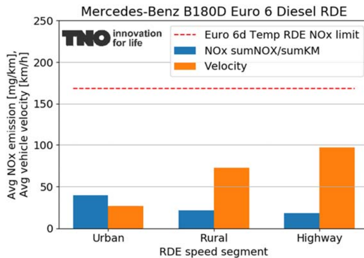
Figure A-43: Average velocities and average NO x emissions in the urban, rural and highway parts of the 'RDE' tests of a Mercedes B180.
