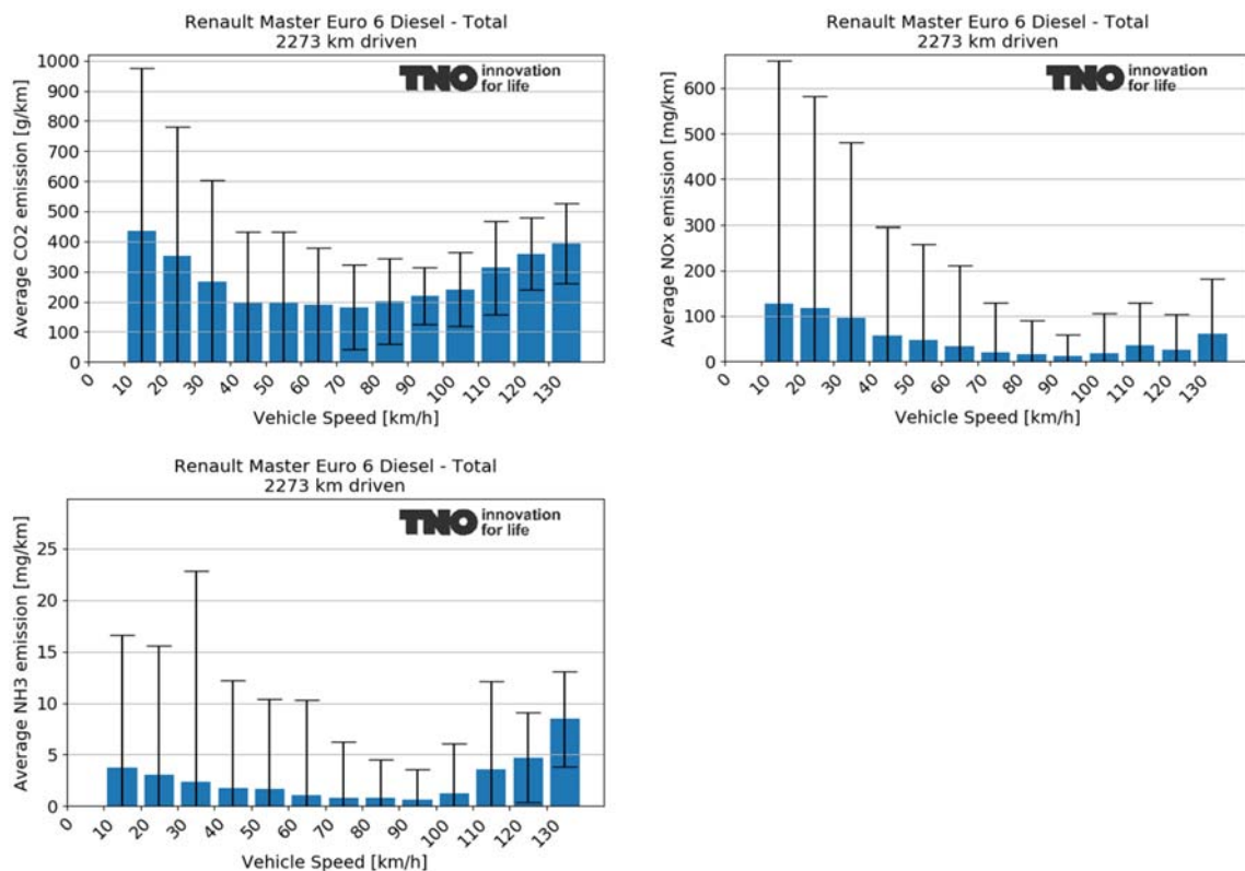
Figure A-51: Average CO 2 , NO x and NH 3 emissions dependent on vehicle speed bin during all driving for a Renault Master
