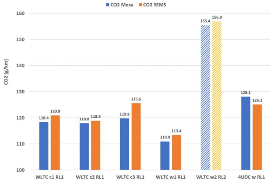
Figure A-24: WLTC and UDC CO 2 test results of a Peugeot Euro 6d-Temp diesel measured with CVS and SEMS. In the WLTC w2 RL2 test the DPF was regenerated.
