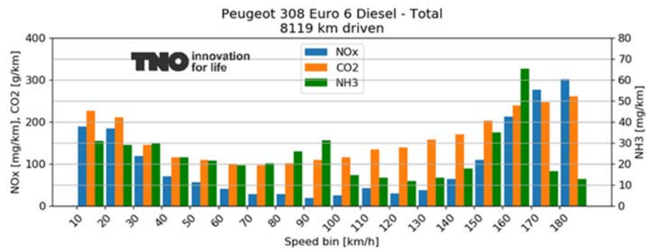
Figure A-61: Binned average emissions of the Peugeot 308 Euro 6d-Temp
