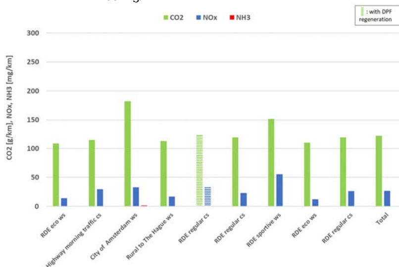
Figure A-45: Average CO 2 , NO x , NH 3 results of the emission test programme of the Mercedes B180.
