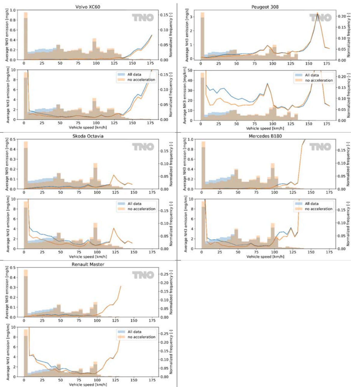
Figure 4-2: Average NH 3 (lines) and frequency distribution (bars) per speed bin for all data and data excluding acceleration (acceleration less than 0.5 m/s 2 , equivalent to 1.8 km/h per second).
