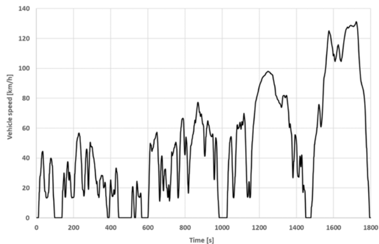
Figure A-1: The Worldwide harmonized Light-duty driving Test Cycle (WLTC_v5).
