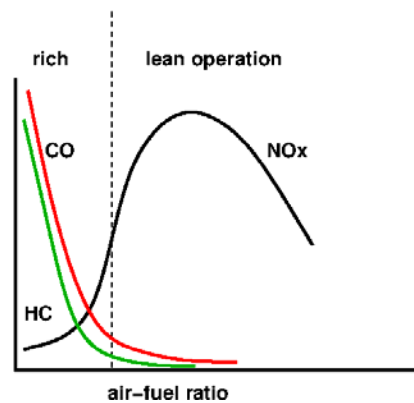
Figure 11-6: The typical emissions of a petrol engine. In lean operation, on the right, NO x emissions are high. In rich operation on the left hydrocarbon and CO emissions are high. In between, at the dashed line, HC, CO, and NO x are produced in the right balance to be converted in a three-way catalyst into harmless products.
