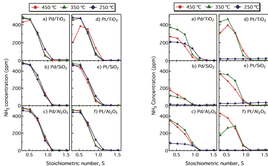
Figure 11-8: Steady-state formation of \text{NH}_3 versus oxygen concentration at 250, 350 and 450 °C (left figure non Water Gas Shift (WGS) assisted and right figure WGS assisted). The gas feed contained 500 ppm NO and 1500 ppm \text{H}_2 while the \text{O}_2 concentration was varied between 0 and 1050 ppm ( S = 0.33 – 1.73 ) in steps of 150 ppm. Air was used as balance and space velocity was 40,000 \text{ h}^{-1} [Adams 2014].
