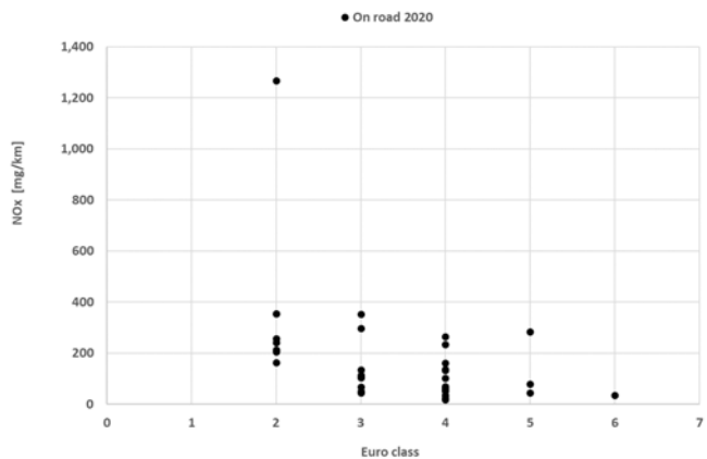
Figure 3-3: Average on road NO x emissions as function of Euro class of 38 petrol vehicles.
