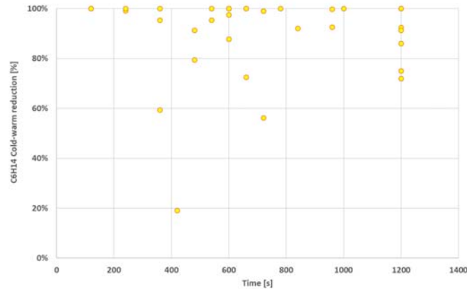
Figure 3-14: C 6 H 14 reduction rates at low idle speed during warming up
