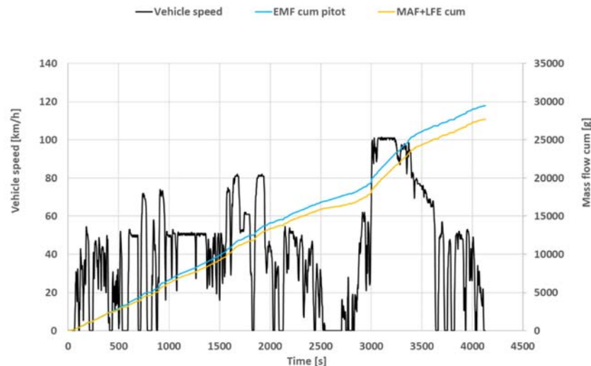
Figure 11-5: Cumulative exhaust mass flows of an on road test of 49 km of the VW Polo Euro 6 petrol measured with the pitot tube (EMF) and the vehicle sensors (MAF + LFE).
