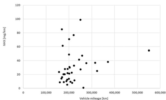
Figure 3-4: Average \text{NH}_3 emissions of road tests as function of the mileages of 38 petrol vehicles.
