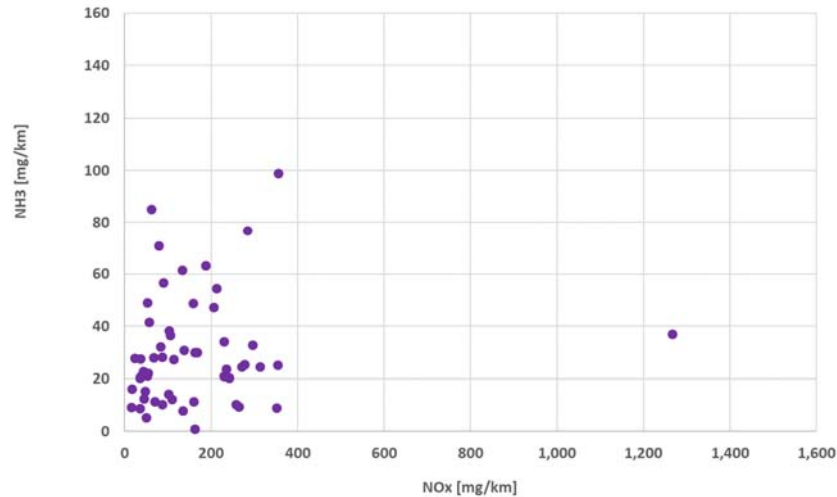
Figure 4-13: Average measured on road \text{NH}_3 emissions as function of average \text{NO}_x emissions of petrol vehicles.
