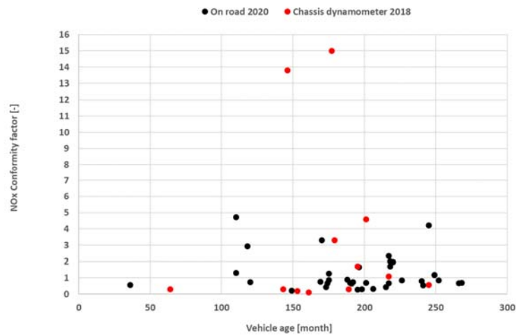
Figure 4-4: NO x conformity factors of 38 + 12 petrol vehicles with high mileages related to vehicle age.
