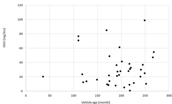
Figure 3-5: : Average on-road \text{NH}_3 emissions as function of vehicle age of 38 petrol vehicles.
